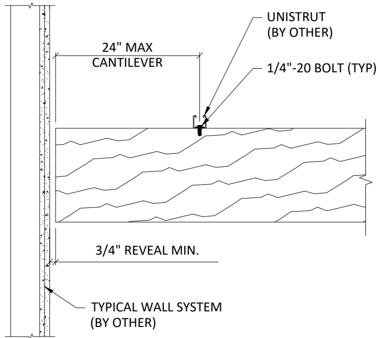
2 PERIMETER CONDITION (SIDE) 1" = 1' 0"
