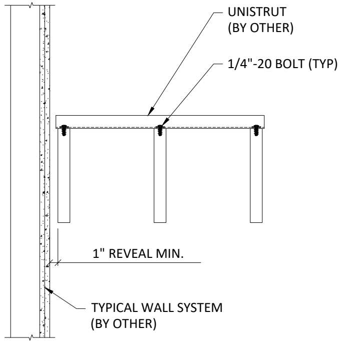
1 PERIMETER CONDITION (FRONT) 1" = 1' 0"
