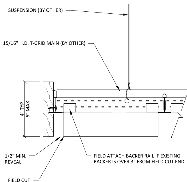
3 TRIM DETAIL 2 3" = 1'-0"
