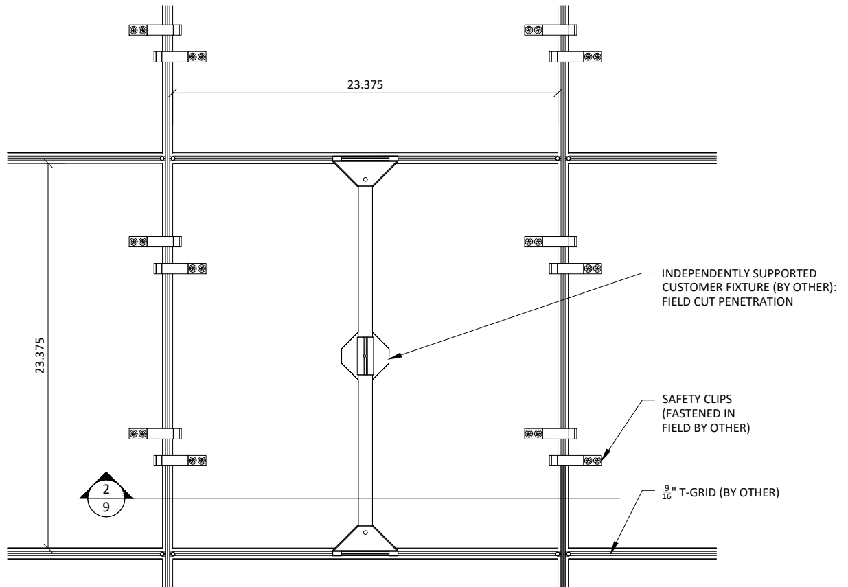
1 DIFFUSER PLAN 9 SCALE: 1 1/2" = 1' 0"
