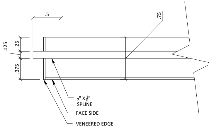
2 SPLINE DETAIL SCALE: 1' 0" = 1' 0"
