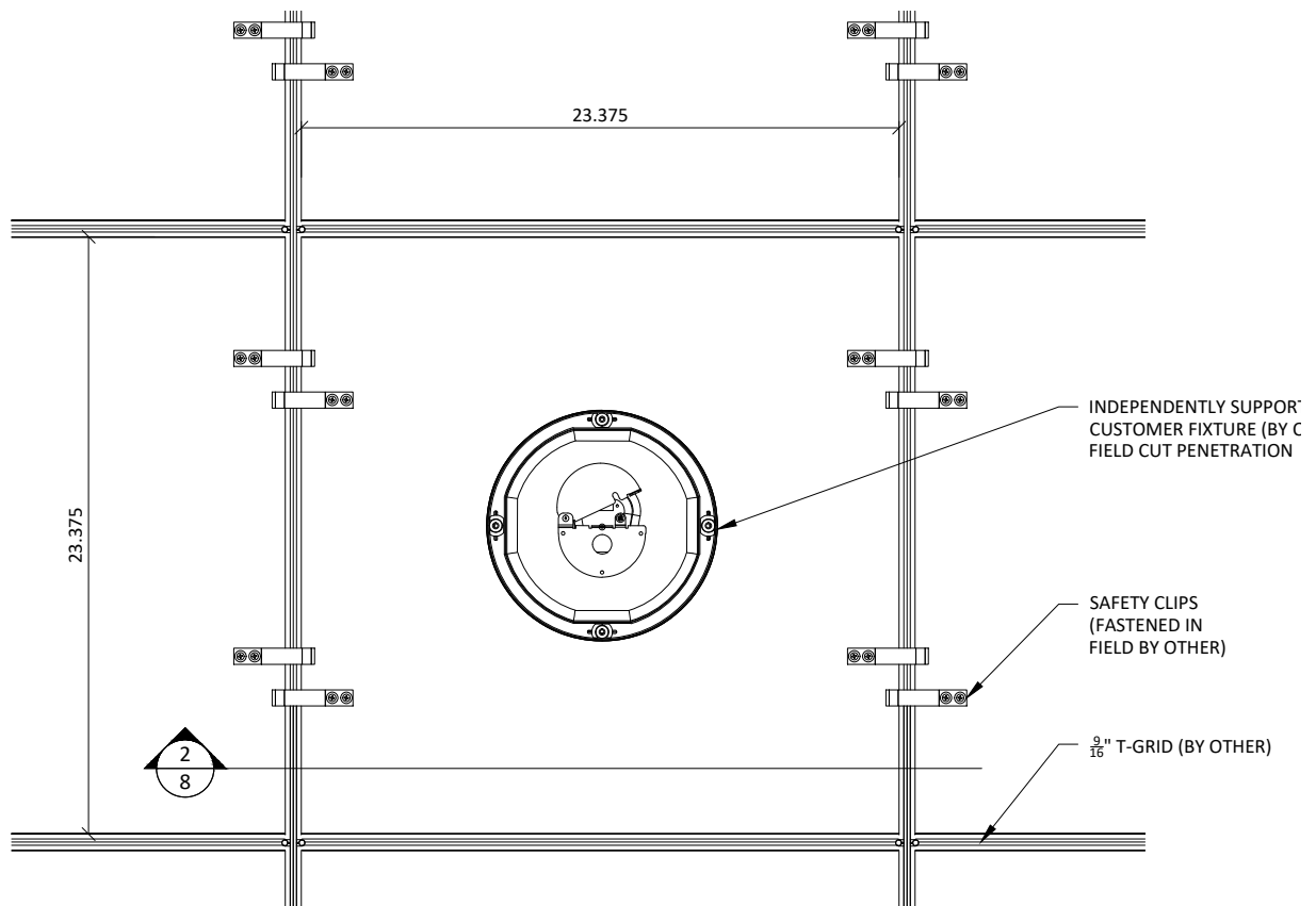
1 RECESSED SPEAKER PLAN SCALE: 1 1/2" = 1' 0"
