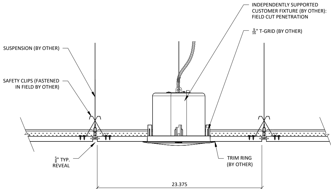
2 RECESSED SPEAKER SECTION SCALE: 1 1/2" = 1' 0"
