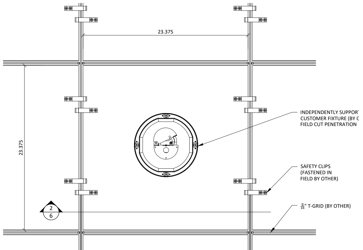
1 CAN LIGHT PLAN SCALE: 1 1/2" = 1' 0"
