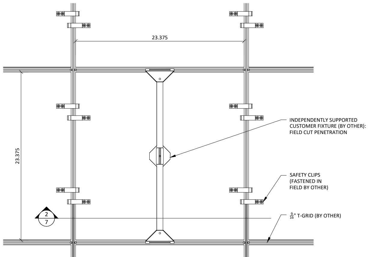
1 PENDANT LIGHT PLAN SCALE: 1 1/2" = 1' 0"
