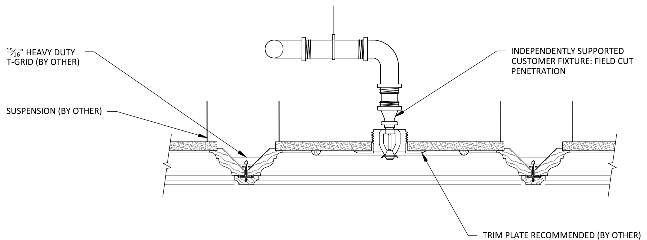
2 SPRINKLER HEAD DETAIL - SECTION VIEW 1 1/2" = 1'-0"
