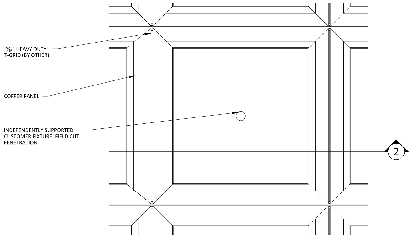
1 SPRINKLER HEAD DETAIL - PLAN VIEW 1 1/2" = 1'-0"
