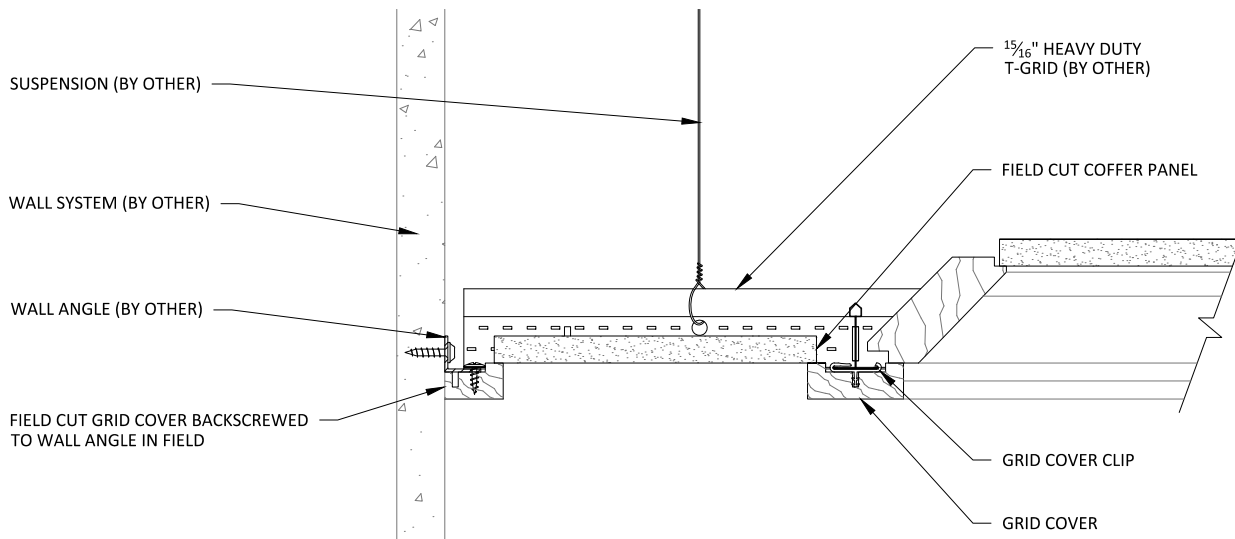
2 TYPICAL PERIMETER CONDITION 3" = 1'-0"
