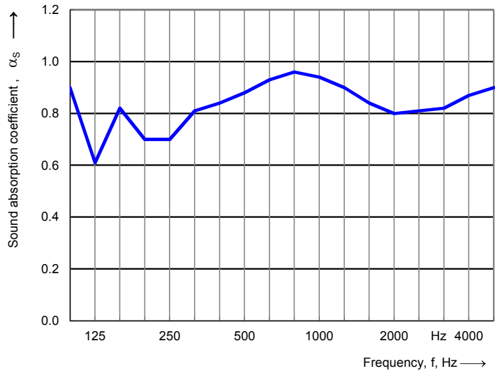
E400 test with Audition 8 (2" backing)
