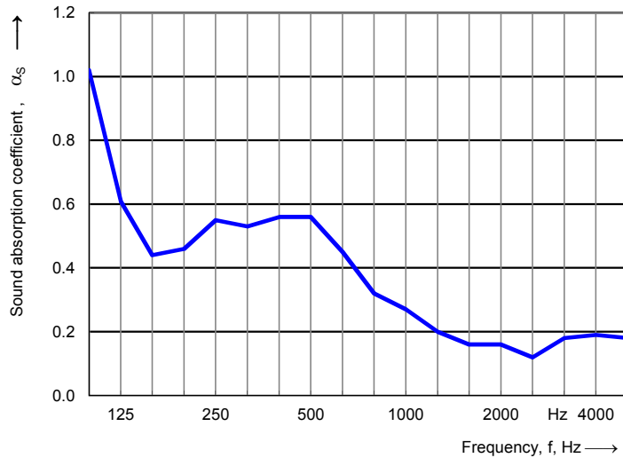
E400 test with 6" Linear Reveal (2-inch backing)
