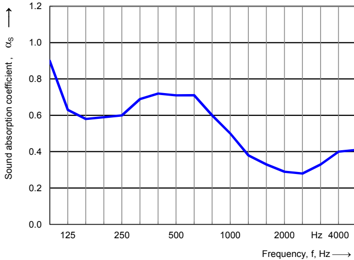
E400 test with 4" Linear Veneer (2-inch backing)
