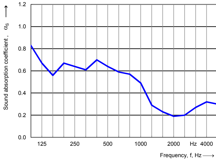
E400 test with 4" Linear Veneer (1-inch backing)
