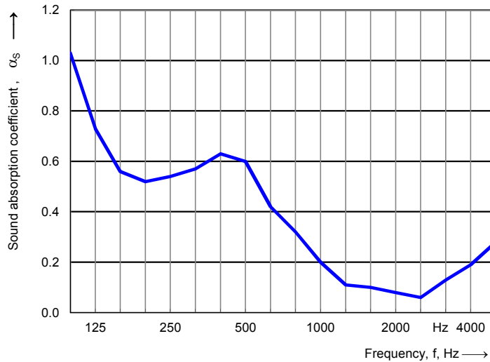
E400 test with 6" Alumiline (1-inch backing)
