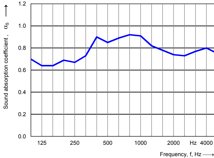
E400 test with Grolle Backered (2-inch backing)
