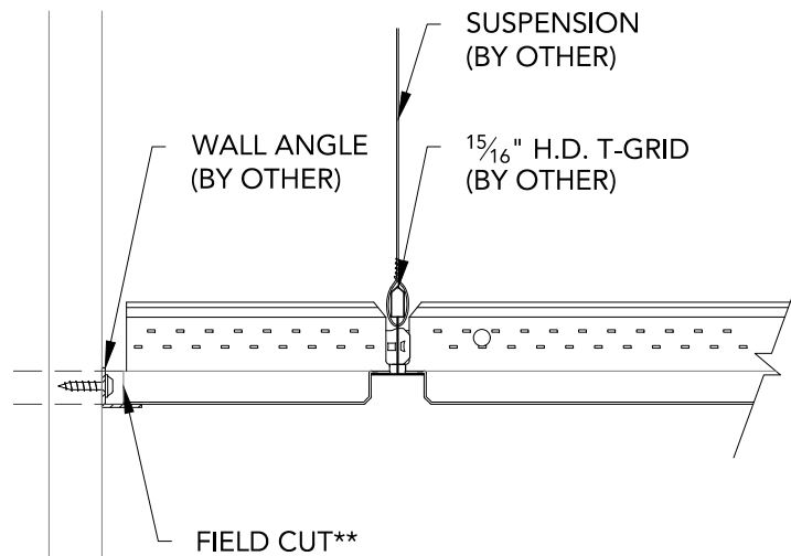
2 FIELD CUT PERIMETER CONDITION 3" = 1'-0"
