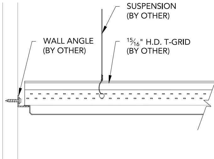
1 TYPICAL PERIMETER CONDITION 3" = 1'-0"
